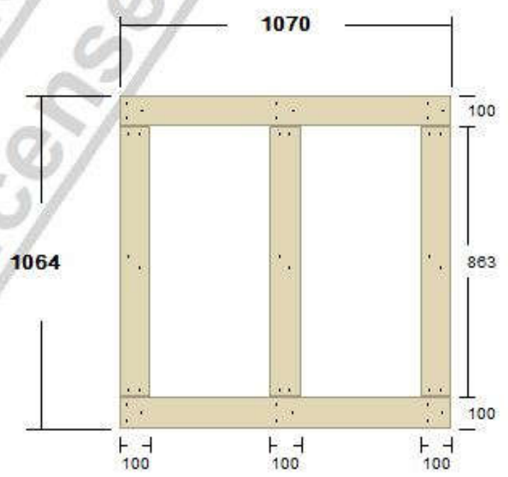
Bottom View
